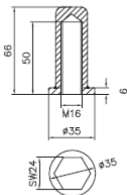
Collar nut M12/M16 Art. No. 2032
